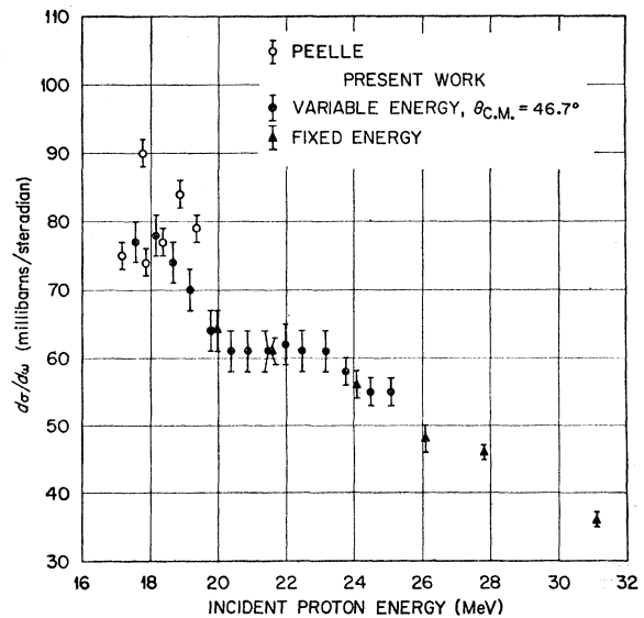
FIG. 4. Differential elastic scattering cross sections at \theta_{c.m.}=46.7^\circ . The data labeled "Pelle" were taken from Ref. 4.
